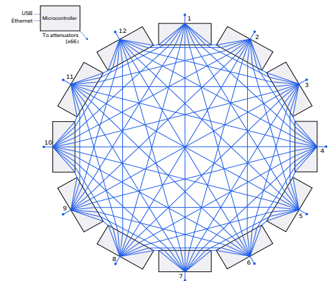
66 internal paths with programmable attenuators on each path
