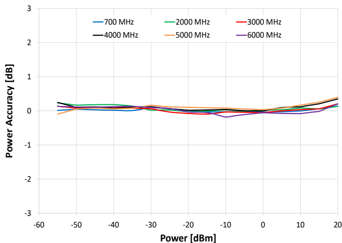
Power Accuracy vs. Output Power
