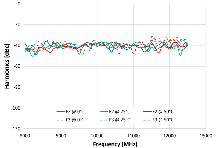
Harmonics vs. Output Frequency @ -40 dBm
