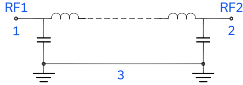
Figure 1. LFHKI-2850+ Functional Diagram
