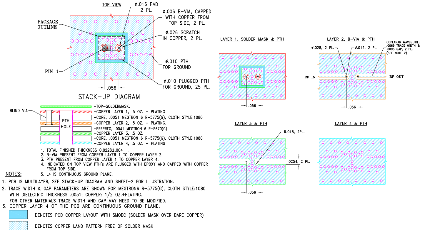
Figure 2. Suggested PCB Layout PL-798
