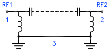
Figure 1. HFHK-1600+ Functional Diagram
