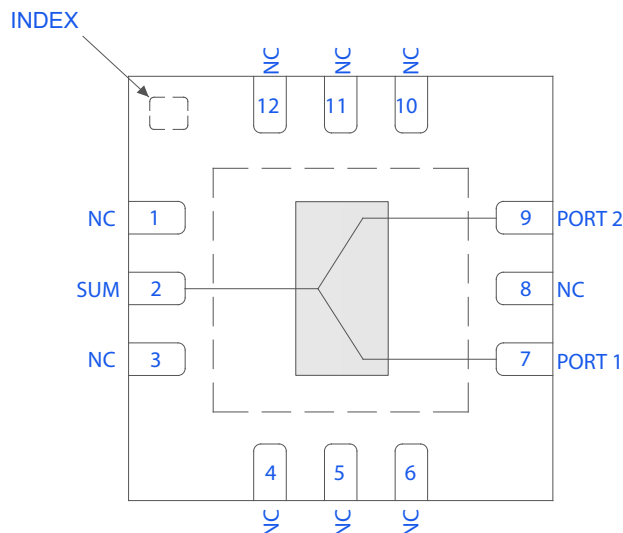
Figure 1. GP2YA+ Functional Diagram
