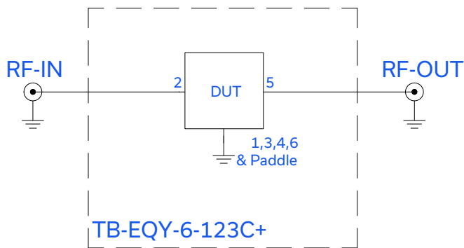
Figure 2. EQY-6-123C+ Evaluation and Application Circuit
