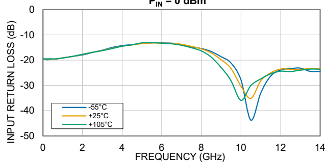
INPUT RETURN LOSS vs. TEMPERATURE
