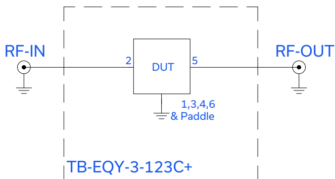
Figure 2. EQY-3-123C+ Evaluation and Application Circuit
