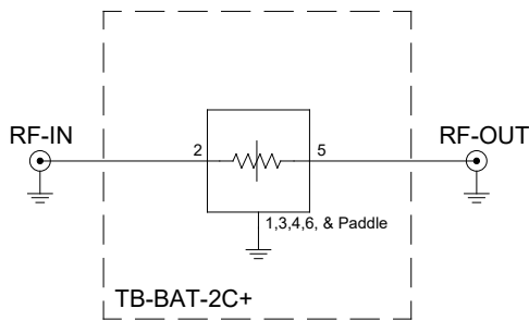
Figure 2. BAT-2+ Characterization and Application Circuit.
