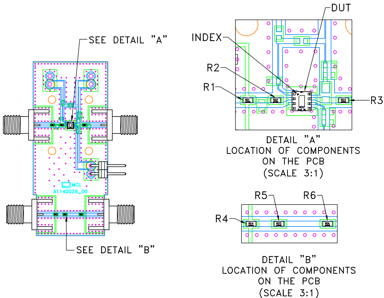
DETAIL "A"
