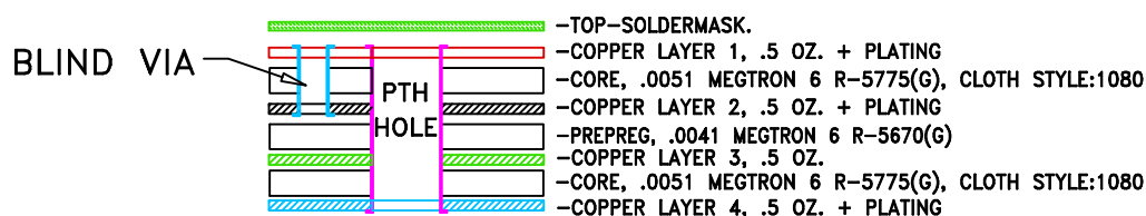
STACK-UP DIAGRAM
