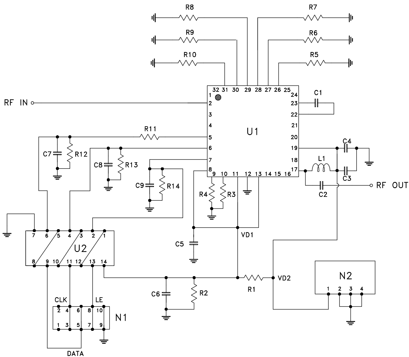
Schematic Diagram
