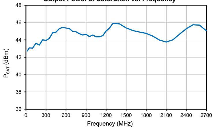
Output Power at Saturation vs. Frequency
