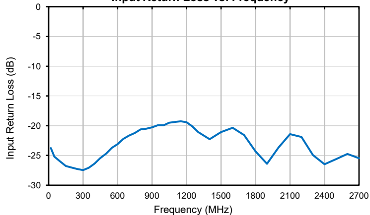
Input Return Loss vs. Frequency
