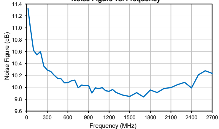
Noise Figure vs. Frequency
