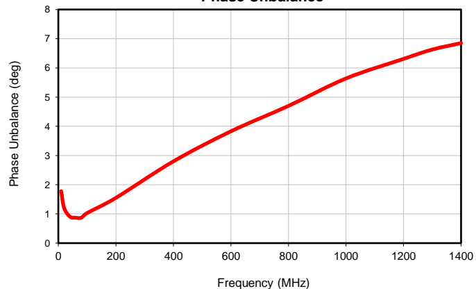
Phase Unbalance
