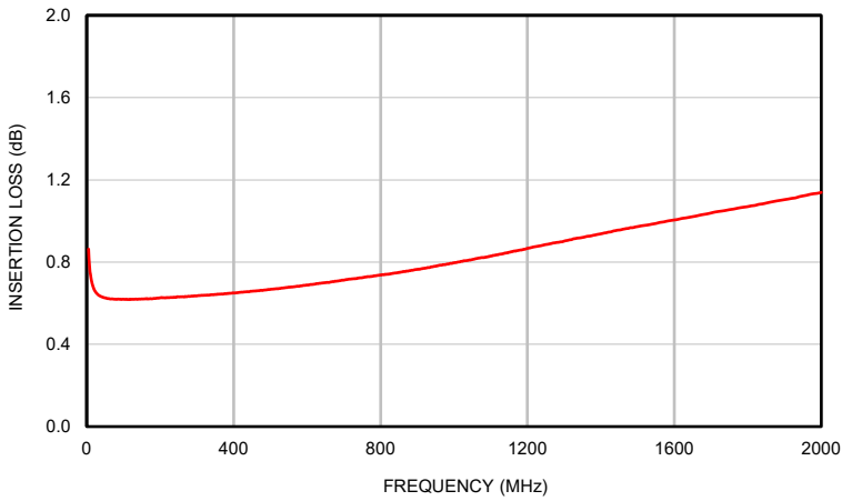
INSERTION LOSS
