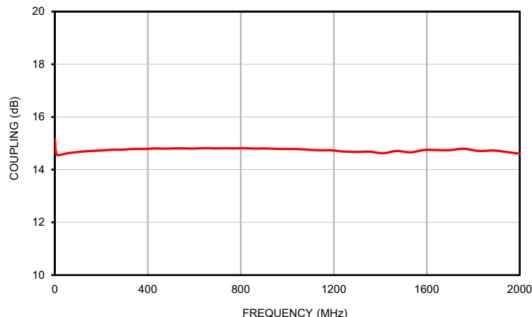
COUPLING
