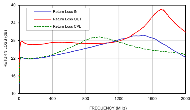
RETURN LOSS
