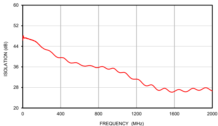
ISOLATION
