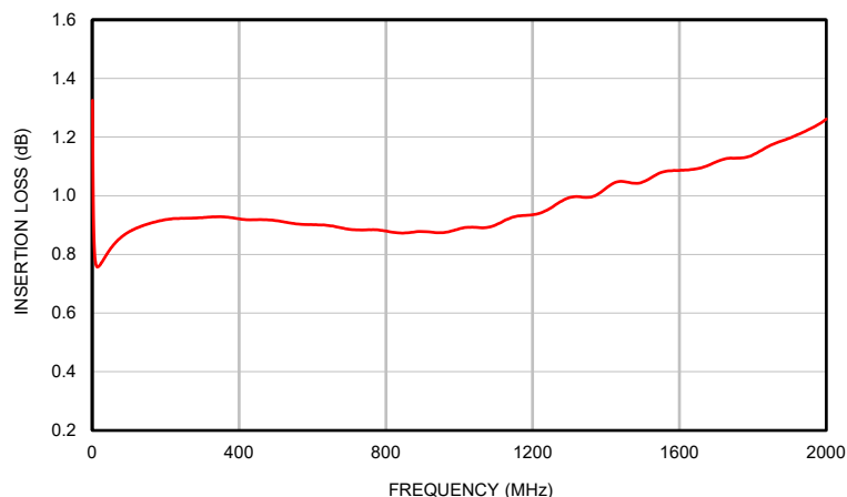
INSERTION LOSS
