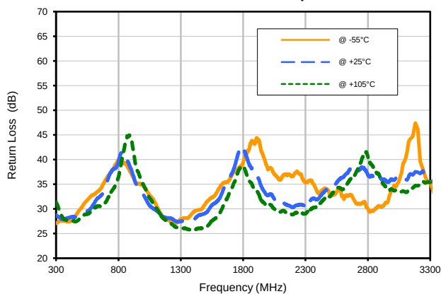
Return Loss Forward vs. Temperature
