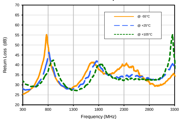
Return Loss In vs. Temperature
