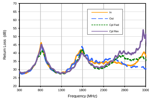
Return Loss
