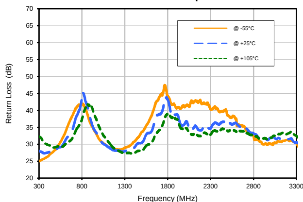
Return Loss Out vs. Temperature
