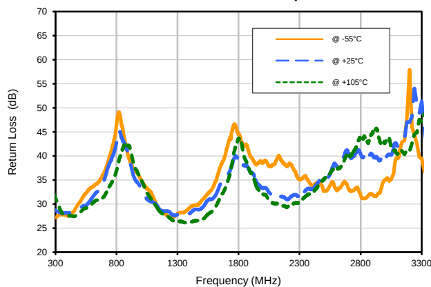
Return Loss Reverse vs. Temperature
