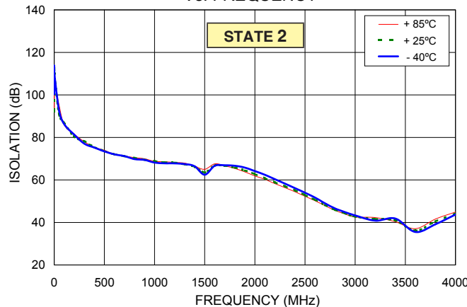
ISOLATION BETWEEN RF1 TO RF2 Vs. FREQUENCY
