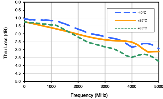
Thru Loss
