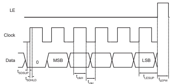
FIGURE 2: SERIAL INTERFACE TIMING DIAGRAM
