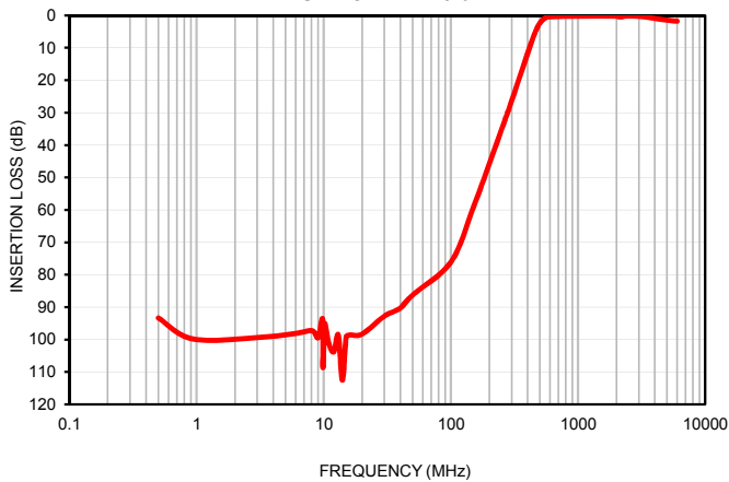
HIGHPASS INSERTION LOSS INPUT POWER = 0 dBm
