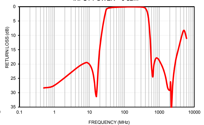
COMMON PORT RETURN LOSS INPUT POWER = 0 dBm
