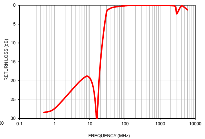
LOWPASS RETURN LOSS INPUT POWER = 0 dBm
