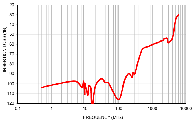
CROSS OVER ISOLATION INPUT POWER = 0 dBm
