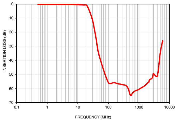
LOWPASS INSERTION LOSS INPUT POWER = 0 dBm
