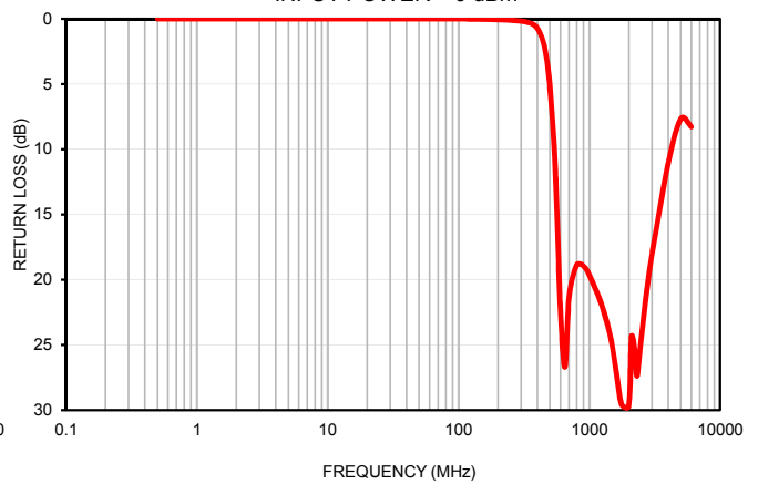
HIGHPASS RETURN LOSS INPUT POWER = 0 dBm
