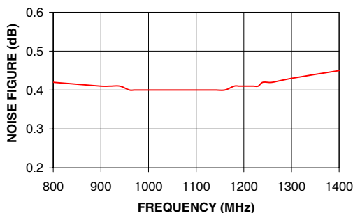
ZX60-1215LN-S+ NOISE FIGURE
