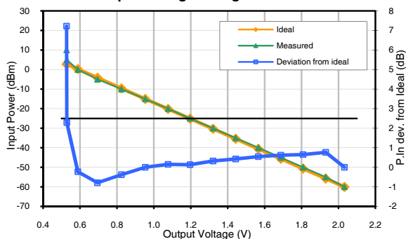
Sensitivity vs. Input Power @+25°C Output Voltage @ Freq 8000MHz
