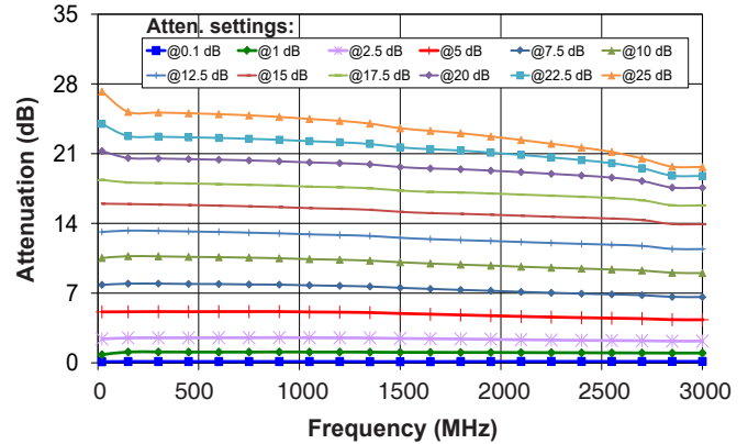
Attenuation relative to I.L. @ +50°C vs. Frequency at selected Atten. settings
