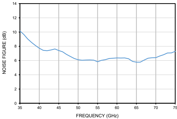
NOISE FIGURE
