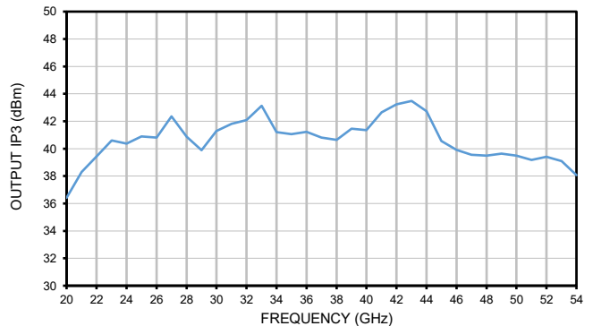
OIP3 @ +25°C
