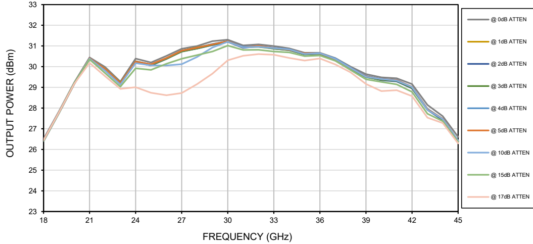
OUTPUT POWER AT 1dB COMPRESSION
