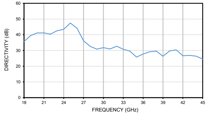
DIRECTIVITY @ +25°C
