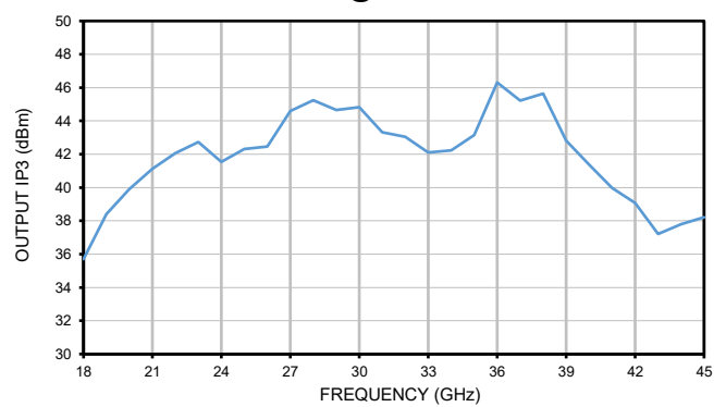
OIP3 @ +25°C
