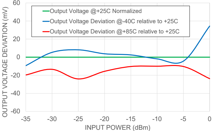
OUTPUT VOLTAGE DEVIATION vs INPUT POWER OVER TEMPERATURE RANGE @ FREQUENCY 20 GHz
