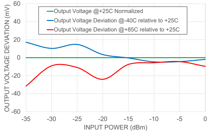
OUTPUT VOLTAGE DEVIATION vs INPUT POWER OVER TEMPERATURE RANGE @ FREQUENCY 100MHz
