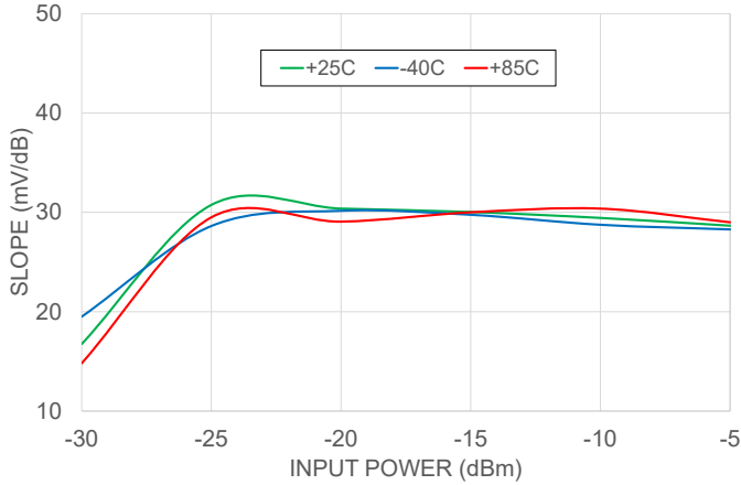
SLOPE Vs INPUT POWER OVER TEMPERATURE RANGE @ FREQUENCY 40 GHz
