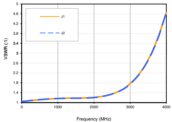
VSWR (J1, J2) Temperature = +25°C
