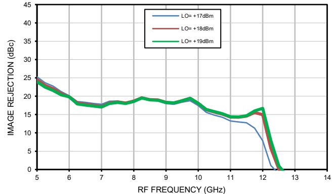
IMAGE REJECTION (DOWNCONVERTER) @ IF = 3000 MHz, IF=LO-RF
