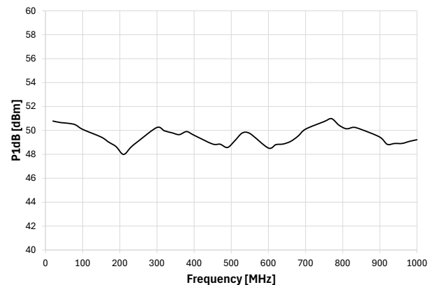
Output Power @ 1dB Compression vs. Frequency
