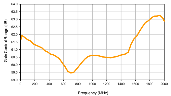
Gain Control Range vs. Frequency @ Vdc=15V
