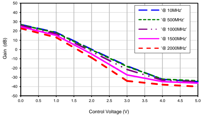
Gain vs. Control Voltage @ Vdc=15V
