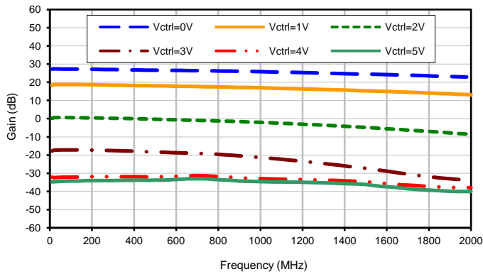
Gain vs. Frequency & Different Vctrl @ Vdc=15V
