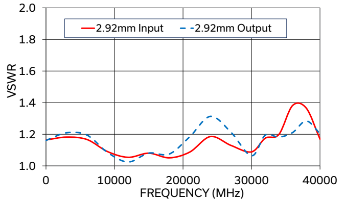
ZEQ-8-44K+ VSWR
