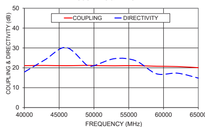
ZCDC20-E40653+ COUPLING & DIRECTIVITY
