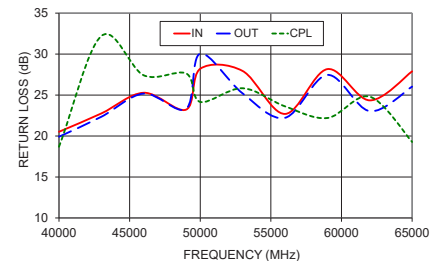
ZCDC20-E40653+ RETURN LOSS
