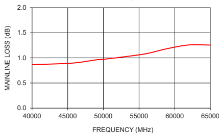
ZCDC20-E40653+ MAINLINE LOSS
