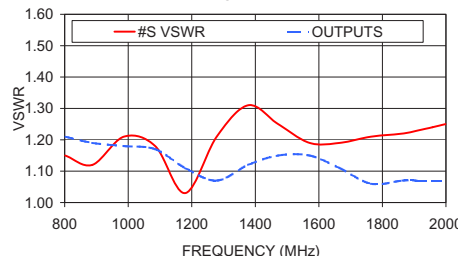
ZB6PD-2+ VSWR
