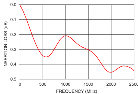
Z7550-BFNF+ INSERTION LOSS
