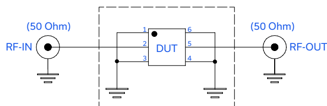
Fig 1. Block diagram of Test Circuit used for characterization, Test board TB-YAT-4A+ Conditions: Attenuation, VSWR: Pin=-10 dBm
