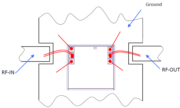
Note: Ground bond wires are optional.
