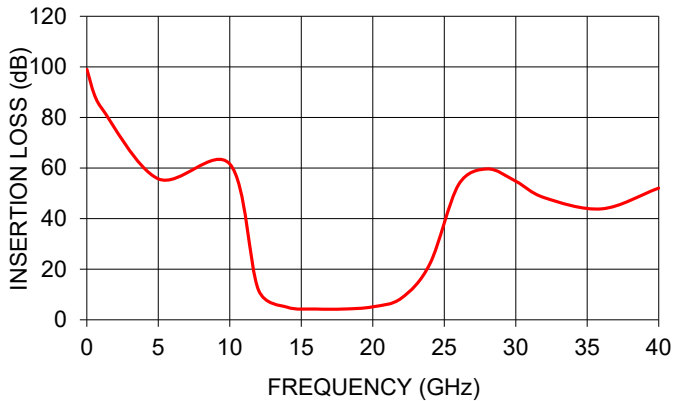
XBF-183+ INSERTION LOSS
