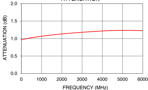
VAT-1A+ ATTENUATION
