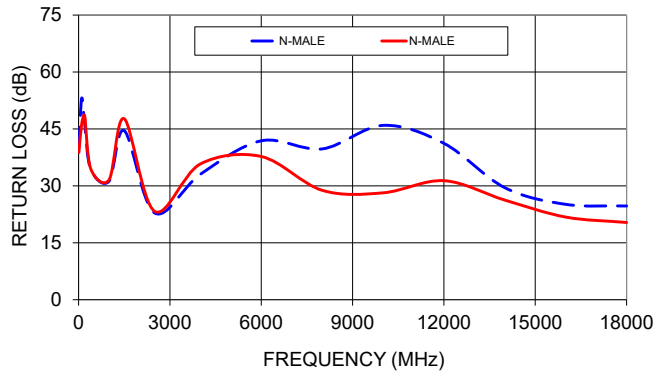
ULC-3FT-NMNM+ RETURN LOSS
