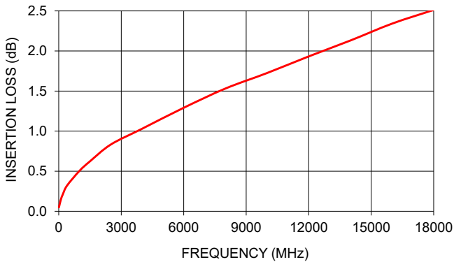
ULC-3FT-NMNM+ INSERTION LOSS
