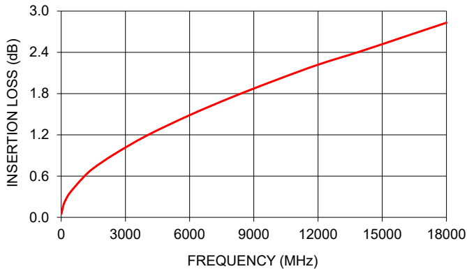
ULC-1M-SMSM+ INSERTION LOSS
