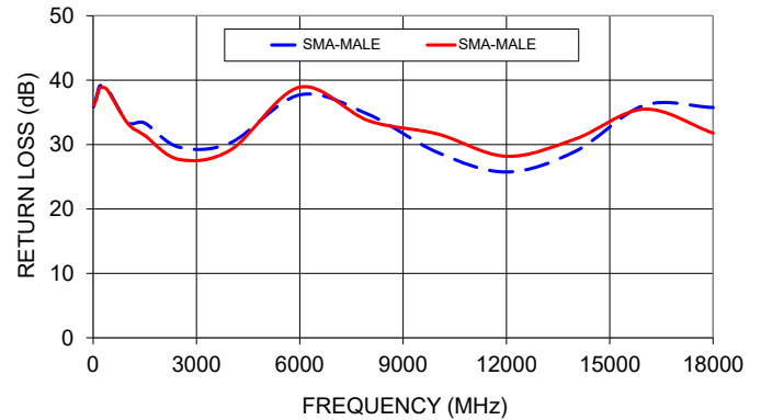
ULC-1M-SMSM+ RETURN LOSS
