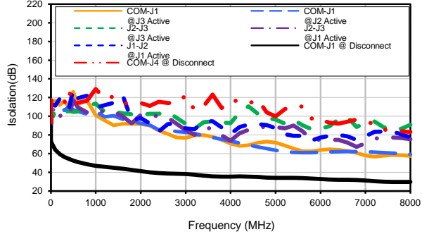
Isolation
