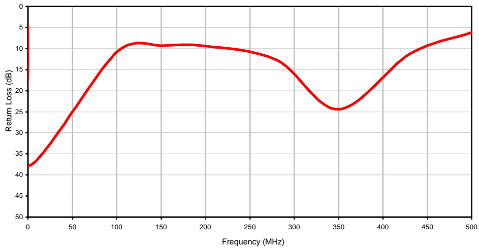
Return Loss
