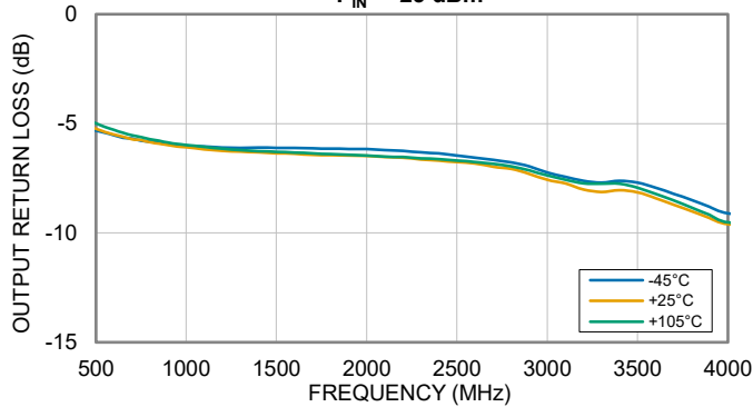
OUTPUT RETURN LOSS vs. TEMPERATURE P_{IN} = -25 dBm
