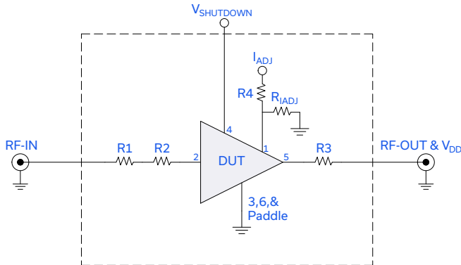
Figure 3. TSS1-43ULN+ Current Adjust Application Circuit
