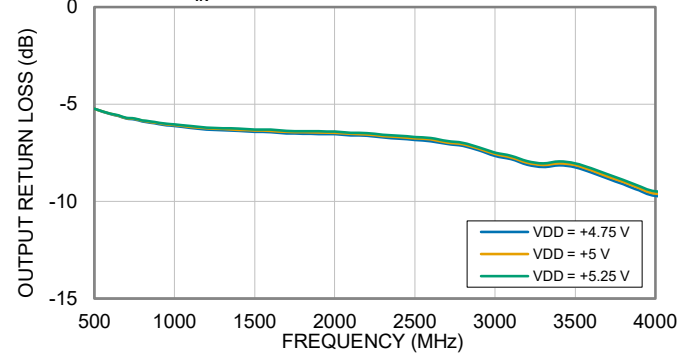
OUTPUT RETURN LOSS vs. DEVICE VOLTAGE ( V_{DD} ) P_{IN} = -25 dBm, TEMPERATURE = +25°C
