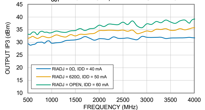
OUTPUT IP3 vs. DEVICE CURRENT ( I_{DD} ) P_{OUT} = +4 dBm/TONE, TEMPERATURE = +25°C
