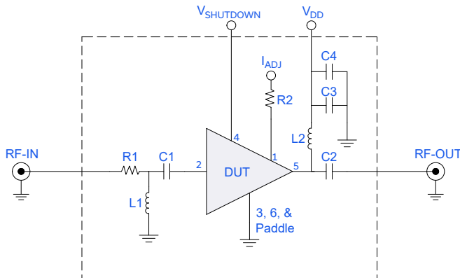
Figure 4. TSS1-43ULN+ 1900-2700 MHz Application Circuit
