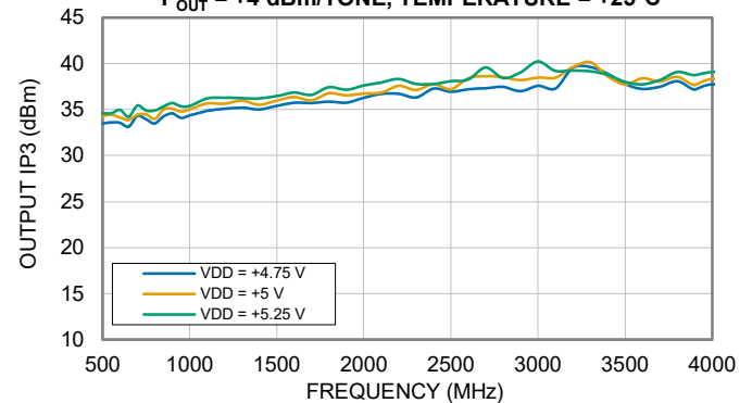
OUTPUT IP3 vs. DEVICE VOLTAGE ( V_{DD} ) P_{OUT} = +4 dBm/TONE, TEMPERATURE = +25°C
