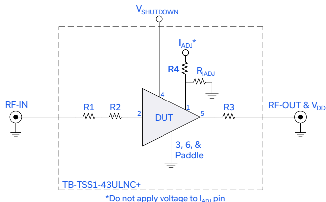
Figure 2. TSS1-43ULN+ Evaluation and Application Circuit
