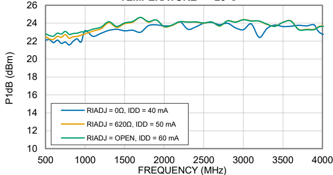
P1dB vs. DEVICE CURRENT ( I_{DD} ) TEMPERATURE = +25°C
