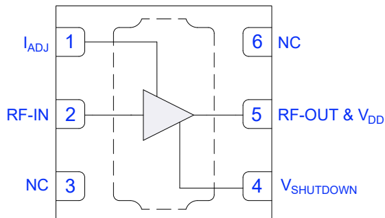
Figure 1. TSS1-43ULN+ Functional Diagram
