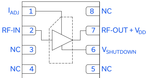
Figure 1. TSS-23ULN+ Functional Diagram
