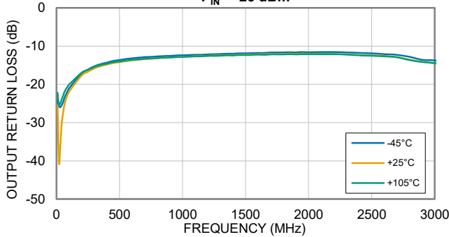
OUTPUT RETURN LOSS vs. TEMPERATURE P_{IN} = -25\text{ dBm}
