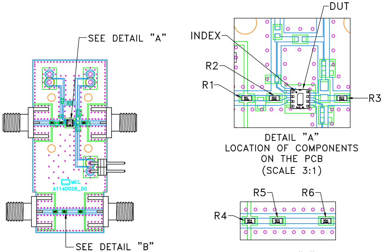
DETAIL "B" LOCATION OF COMPONENTS ON THE PCB (SCALE 3:1)
