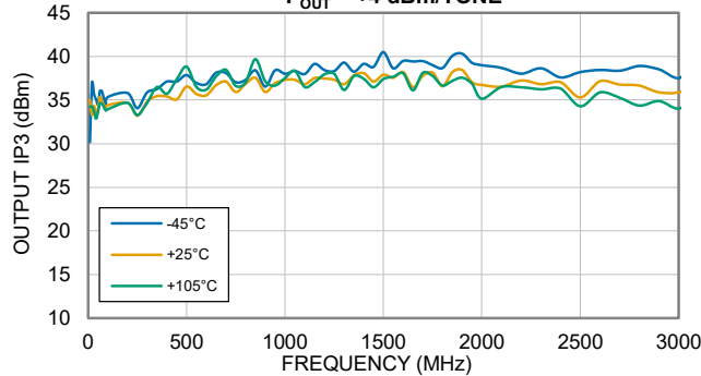
OUTPUT IP3 vs. TEMPERATURE P_{OUT} = +4\text{ dBm/TONE}
