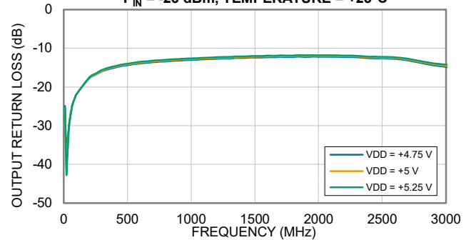
OUTPUT RETURN LOSS vs. DEVICE VOLTAGE ( V_{DD} ) P_{IN} = -25\text{ dBm} , TEMPERATURE = +25°C
