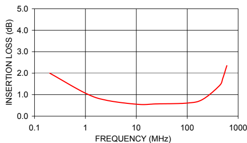
TMO-4-2+ INSERTION LOSS
