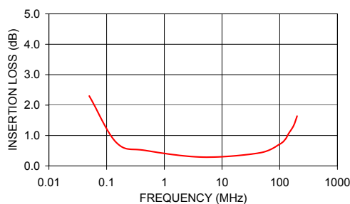
TMO-1-1T+ INSERTION LOSS
